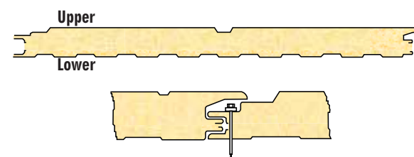
SIP-2002- Zep Wall Panels (Concealed Fastner-3 Profile)
