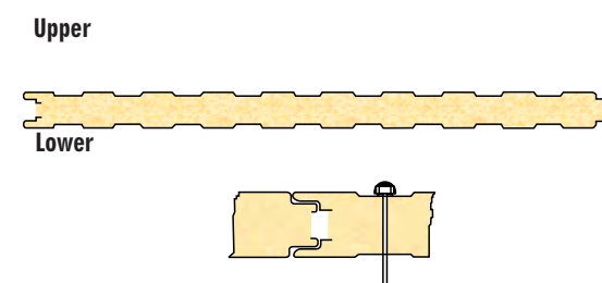
SIP-2003- Zep Wall Panels (External Fastners)
