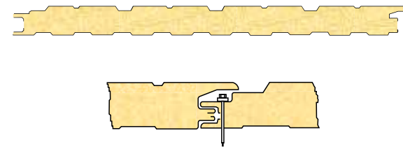
SIP-2001- Zep Wall Panels (Concealed Fastner-Single Profile)
